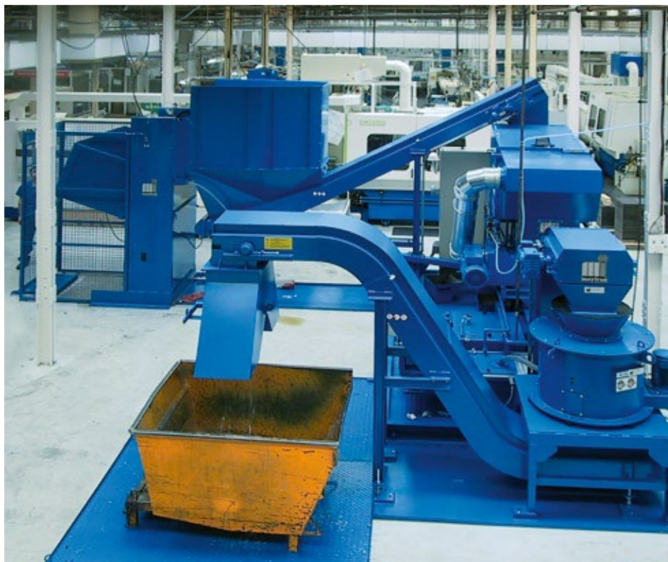
Swarf pressing system comprised of the following components: centrifuge, swarf crusher, conveyor and container loading
